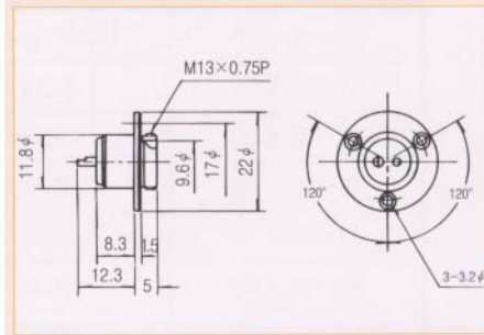
● RECEPTACLE (R)
