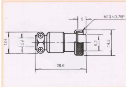
● PLUG (P)
